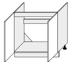
D8Z/80 800/820/500
