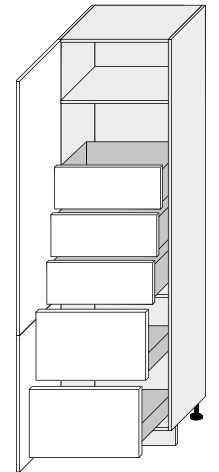
D14/DL/60/207-ST 600/2070/565
