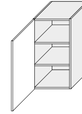
W2/40 400/720/300
