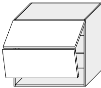
W8B/80 AVENTOS 800/720/325
