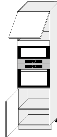
DRU 60/207 600/2070/565
