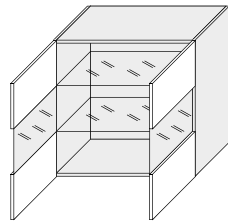
WESZ80/WE1S80 800/720/325
