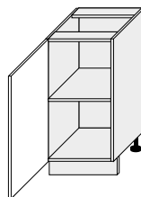
D1D/40 400/820/500
