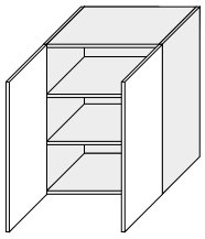
W3/60 600/720/325
