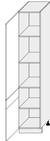
DEPK/40 400/2070/565
