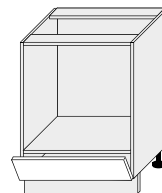
DEP/60 600/820/500
