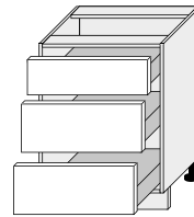
D3E/60 600/820/500
