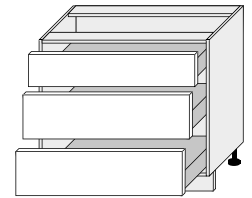
D3M/90 900/820/500
