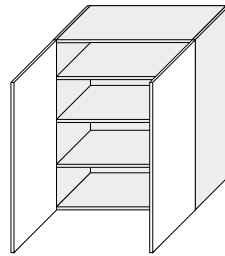
W4/80 800/960/325
